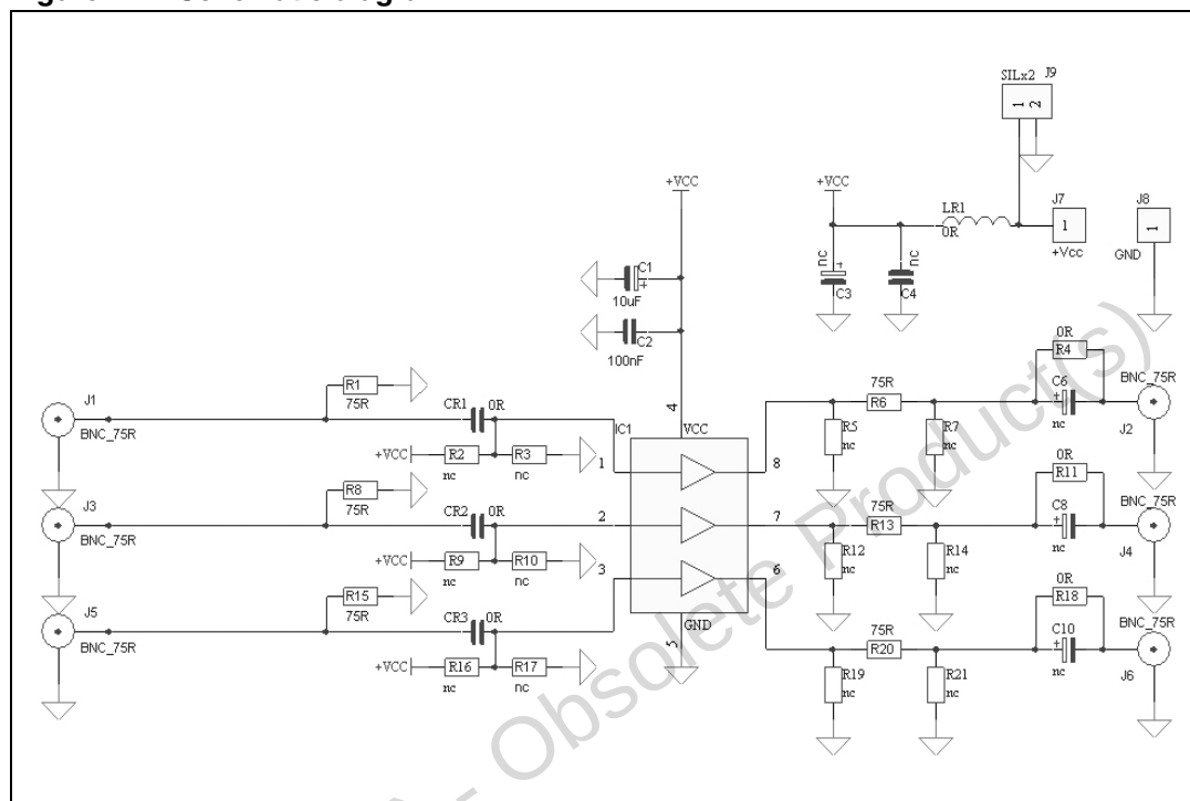
Figure 1. Schematic diagram
